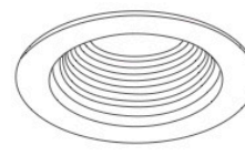
Baffle Trim 4 7/8" O.D. Includes 3-Optic Lens (14°, 24°, 36°)
