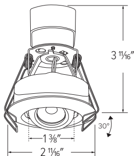
E1L32 - 1" ROUND GIMBAL 30° ADJUSTABILITY
