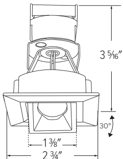
E1L22 - 1" SQUARE PULL DOWN 30° ADJUSTABILITY
