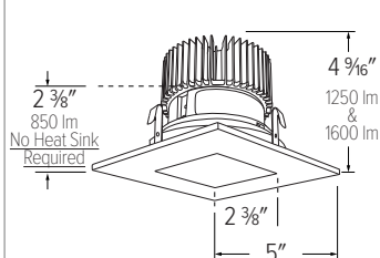
E417C - 4" SQ/SQUARE REFLECTOR
