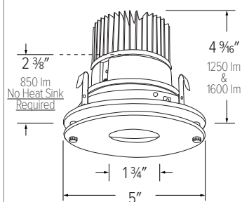
E412C - 4" ROUND DROP GLASS
