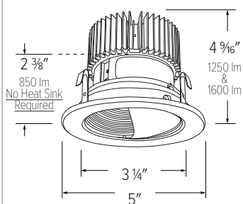
E411C - 4" ROUND WALL WASH
