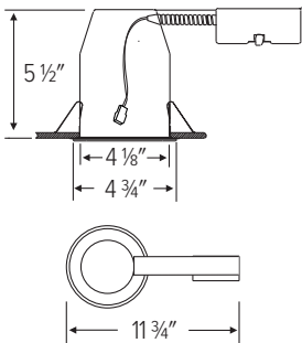
E4LRC08ICA / E4LRC / 08 / 12 / 16 4" REMODEL LED HOUSING
