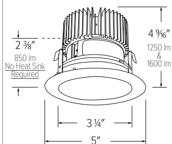
E410C - 4" ROUND REFLECTOR
