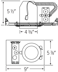
E4LC08ICA / E4LC08 / E4LC12 4" NEW CONSTRUCTION LED HOUSING
