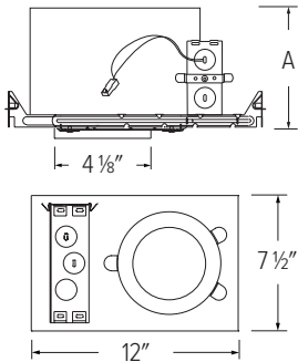
E4LC12ICA / E4LC16ICA 4" NEW CONSTRUCTION LED ICA DOUBLE WALL HOUSING
