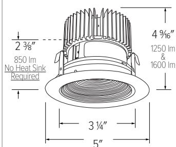
E414C - 4" ROUND BAFFLE
