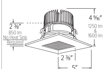
E415C - 4" SQUARE BAFFLE
