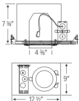
E4FH08ICA 4" NEW CONSTRUCTION LED HOUSING 2-HOUR FIRE RATED
