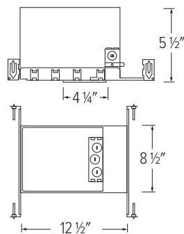
E4AJC08ICAD2 / E4AJC12ICAD2 4" NEW CONSTRUCTION FOAM INSULATED R60 LED HOUSING
