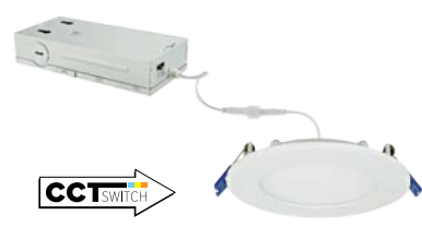
0-10V Ultra Slim LED Panel Lights with 5-CCT Switch
