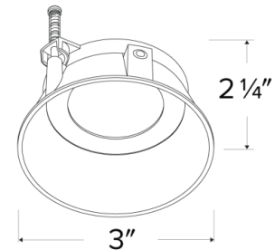
EL3WCRW - White Adaptor with Mounting Clips
