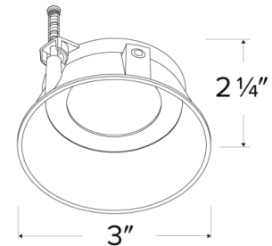
EL3WCRW - White Adaptor with Mounting Clips
