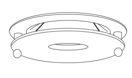
Reflector with Suspended Glass 4 7/8" O.D. Includes 3-Optic Lens (14°, 24°, 36°)
