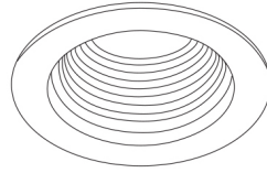
Baffle Trim with Regressed Lens 4 7/8" O.D.
